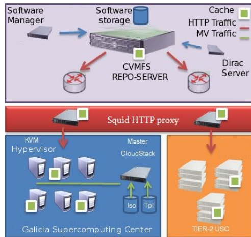
Figure 3.6: CernVM-FS repository and Architecture Deployment.
