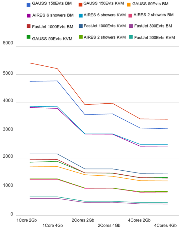
Figure 3.13: Walltime mean values of all HEP-Software in Virtualized and Non-virtualized nodes
