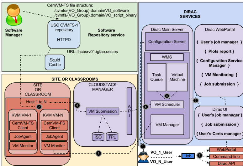
Figure 5.1: CloudStack prototype design in the Formiga-Cloud project.
