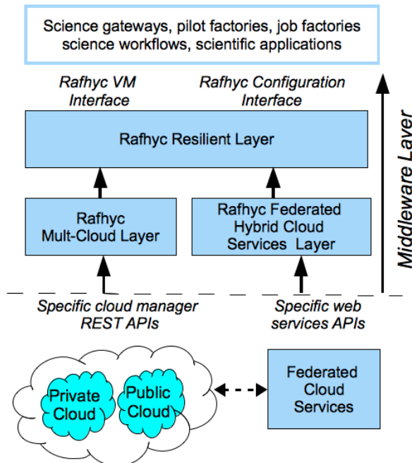
Figure 4.12: Rafhyc Overall Architecture.
