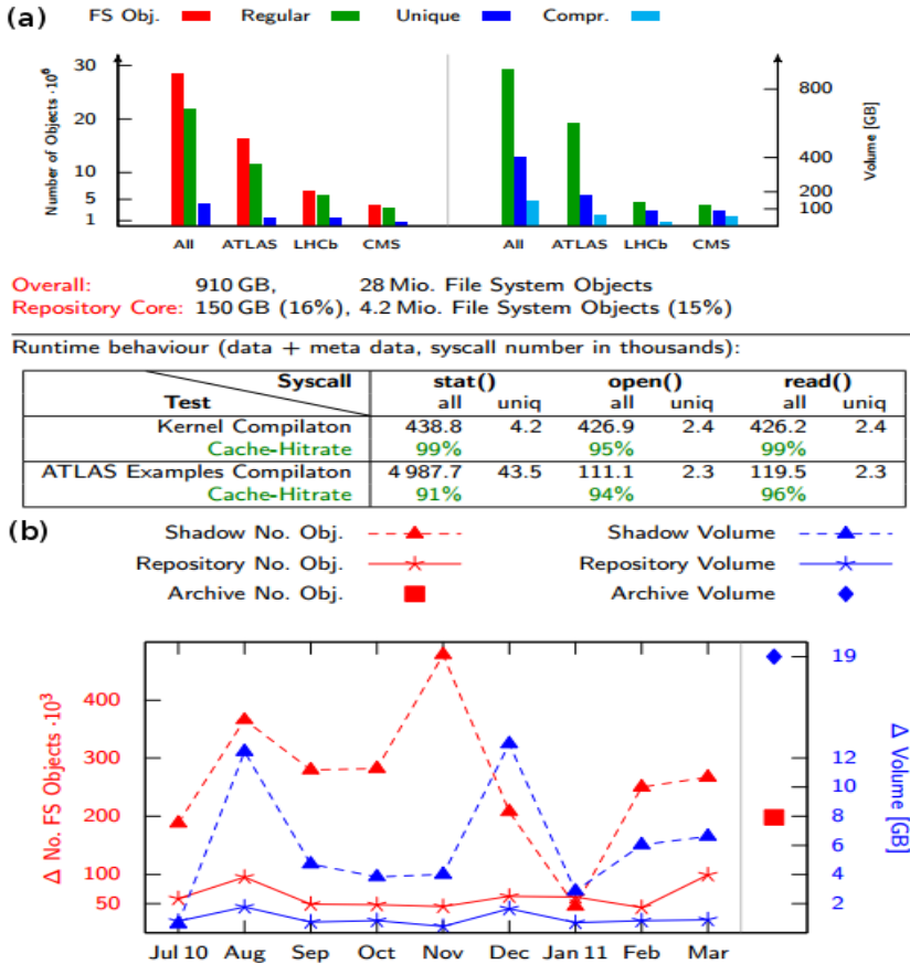
Figure 3.5: Features of the LHC experiments software.
